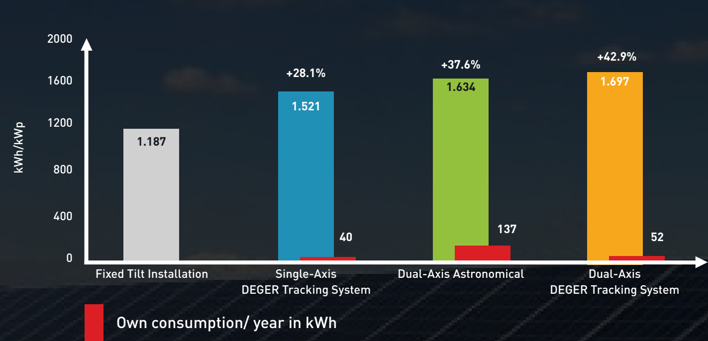
COMPARATIVE MEASUREMENTS IN 2012 IN SOLAR PARK REXINGEN
